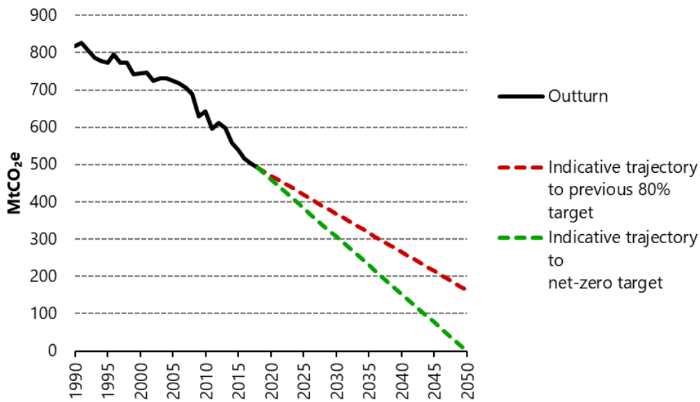
Figure 4. UK Greenhouse Gas emission reductions required to meet Net Zero. 15
